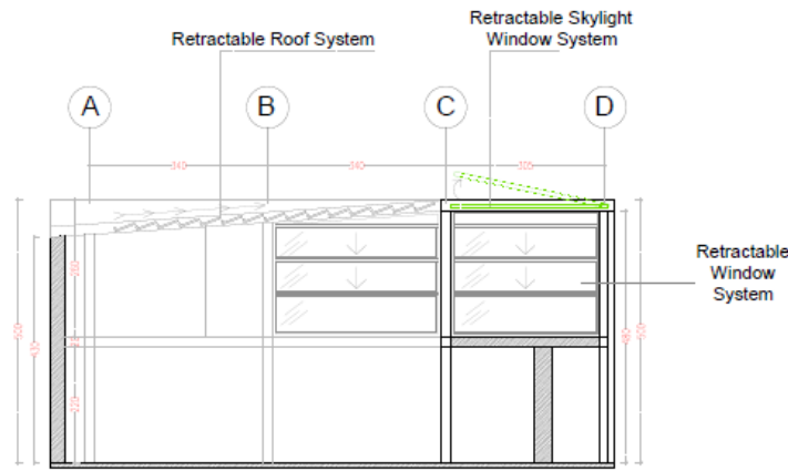
BB SECTION
