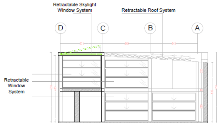
CC SECTION
