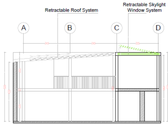
AA SECTION
